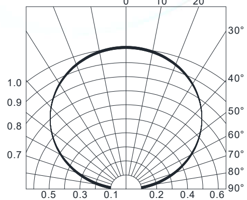
Fig.4-Radiation Diagram T_a=25^\circ\text{C}
