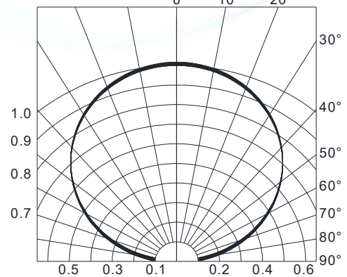
Fig.4-Radiation Diagram T_a=25^\circ\text{C}
