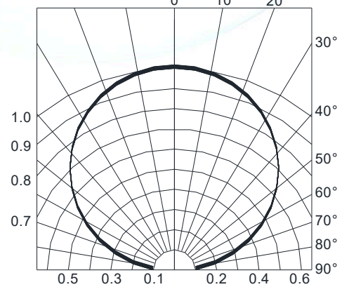
Fig.4-Radiation Diagram T_a=25^\circ\text{C}
