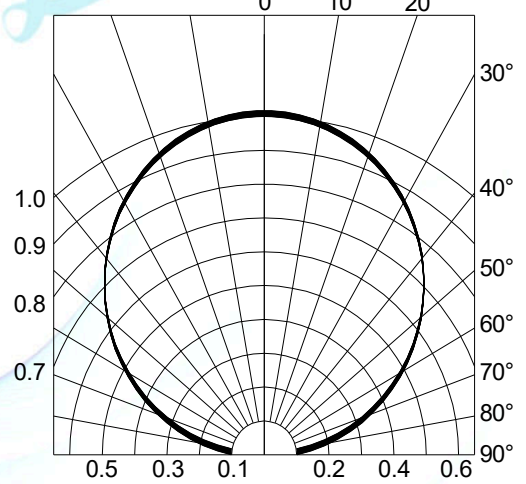
Fig.4-Radiation Diagram T_a=25^{\circ}\text{C}
